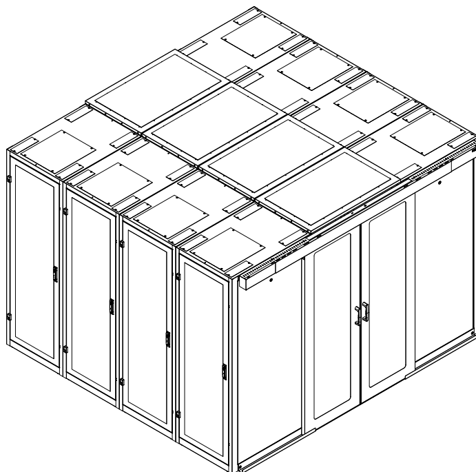
Typical COLD AISLE CONTAINMENT configuration
